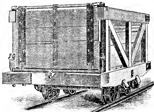
Fig. 32. MINE CAR, END DUMP, BUILT BY BLOOMSBURG CAR COMPANY.
